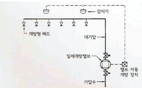
일제살수식(Deluge system)
