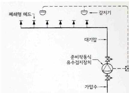
준비작동식(Preaction system)
